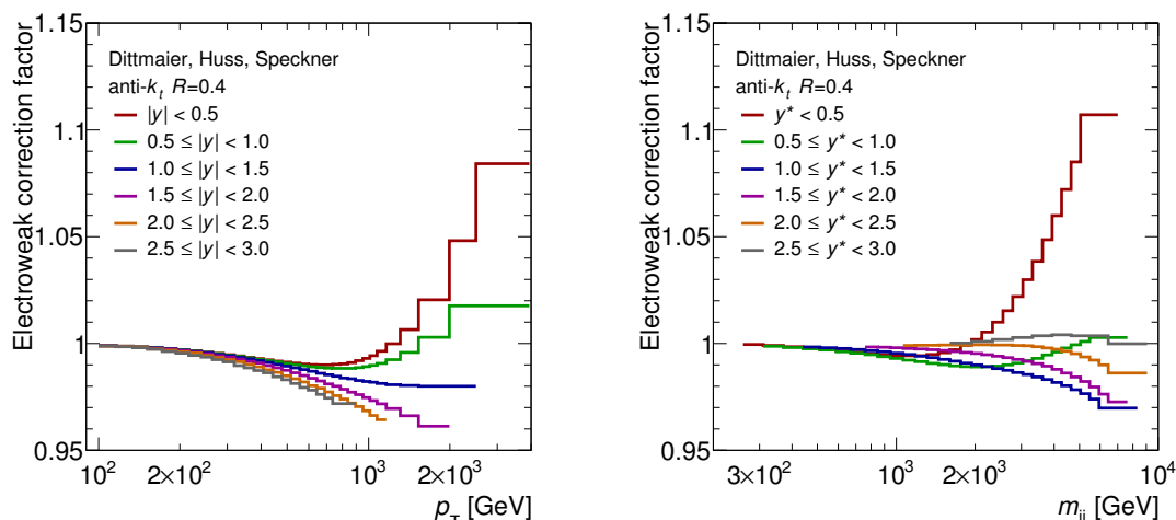
Figure 4. Electroweak correction factors for the inclusive jet (dijet) cross-section as a function of the jet p_T ( m_{jj} ) for all |y| ( y^* ) bins.
