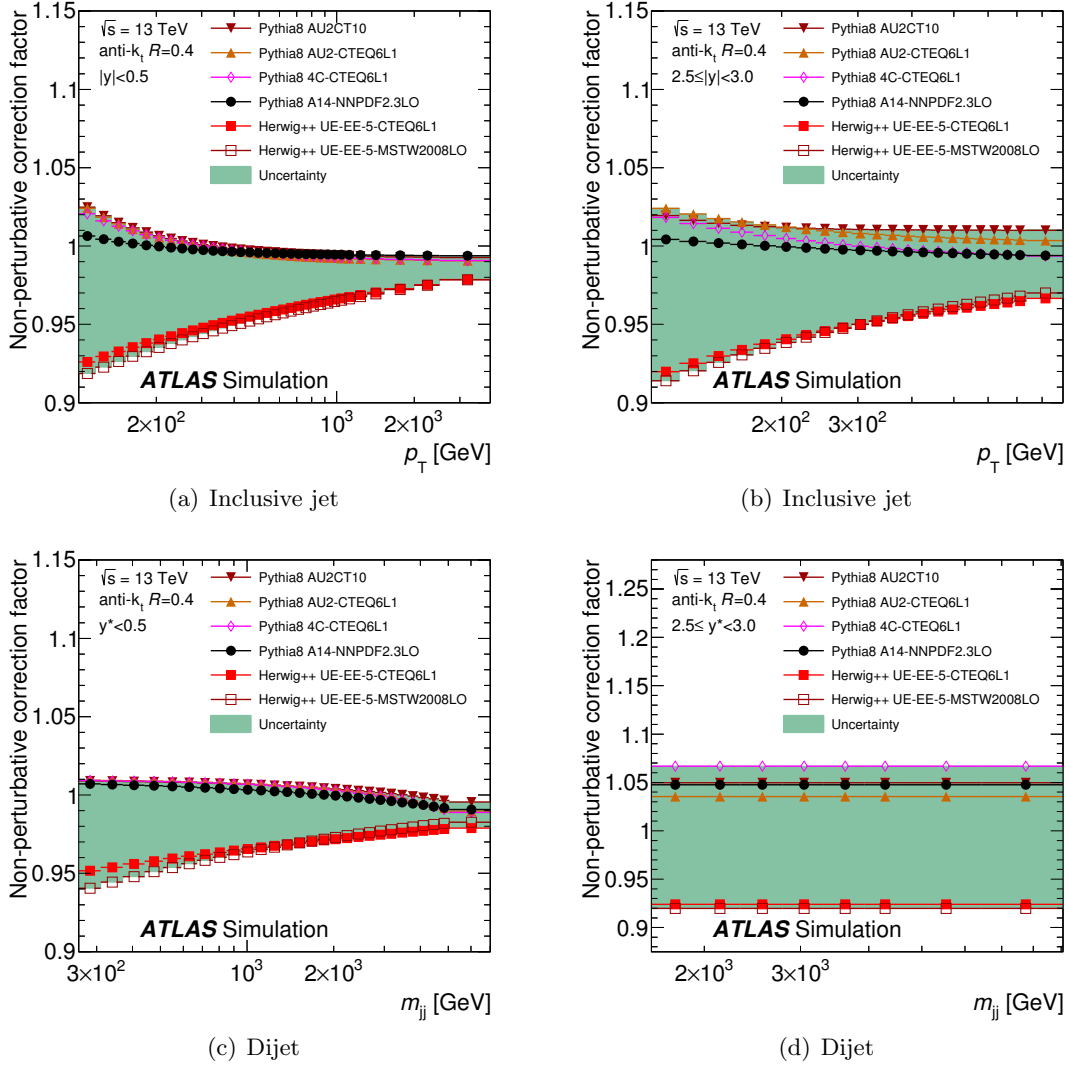
Figure 3. Non-perturbative correction factors for the (inclusive jet, dijet) NLO pQCD prediction as a function of (jet p_T , m_{jj} ) for ((a), (c)) the first (rapidity, y^* ) bin and for ((b), (d)) the last (rapidity, y^* ) bin. The corrections are derived using PYTHIA 8 with the A14 tune with the NNPDF2.3 LO PDF set. The envelope of all MC configuration variations is shown as a band.
