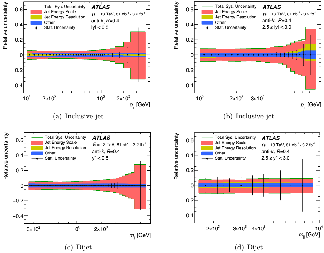
Figure 1. Relative systematic uncertainty for the inclusive jet cross-section as a function of the jet p_T for the first and last rapidity bins ((a) and (b) respectively) and for the dijet cross-section as a function of m_{jj} for the first and last y^* bins ((c) and (d) respectively). The individual uncertainties are shown in different colours: the jet energy scale, jet energy resolution and the other uncertainties (jet cleaning, luminosity and unfolding bias). The total systematic uncertainty, calculated by adding the individual uncertainties in quadrature, is shown as a green line. The statistical uncertainty is shown as vertical black lines.
