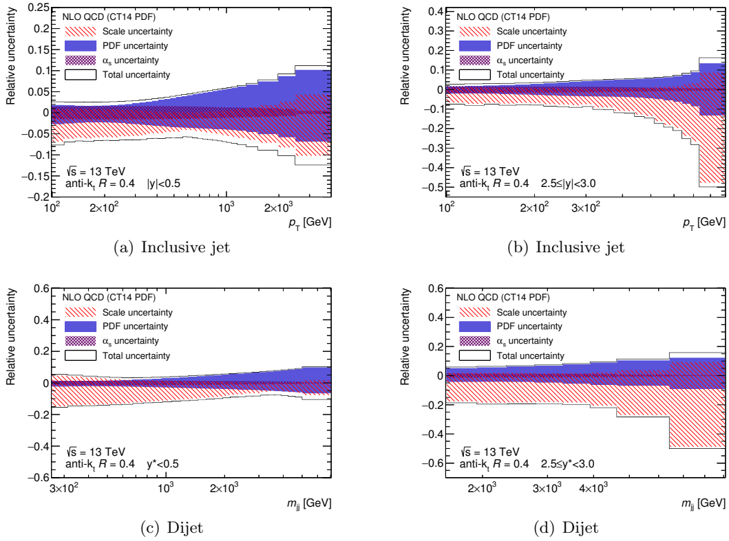
Figure 2. Relative NLO QCD uncertainties in the jet cross-sections calculated using the CT14 PDF set. Panels a,b (c,d) correspond respectively to the first and last |y| ( y^* ) bins for the inclusive jet (dijet) measurement. The uncertainties due to the renormalisation and factorisation scale, the \alpha_s , the PDF and the total uncertainty are shown. The total uncertainty, calculated by adding the individual uncertainties in quadrature, is shown as a black line.
