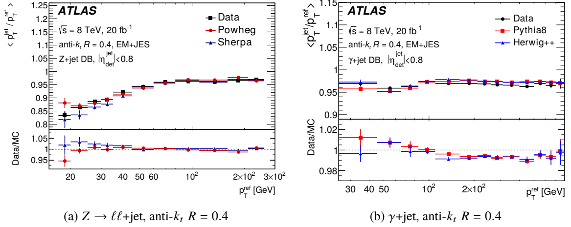
Figure 22: R_{\text{DB}} for anti- k_t jets with R = 0.4 and calibrated with the EM+JES scheme from the (a) Z+jet and (b) \gamma +jet analyses in the data and for two MC simulations. Only statistical uncertainties are shown.
