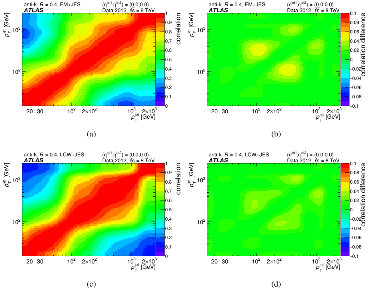
Figure 43: The (a,c) JES correlation matrix and (b,d) difference between the full correlation matrix and that derived from a reduced number (6) of absolute in situ uncertainty components for anti- k_t , R = 0.4 jets calibrated with the (a,b) EM+JES and (c,d) LCW+JES schemes.
