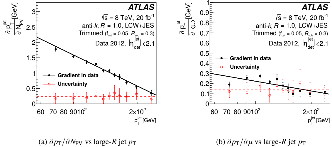
Figure 32: The gradients (a) \partial p_T / \partial N_{PV} and (b) \partial p_T / \partial \mu extracted in \gamma +jet data (filled circles) and the difference of the gradients measured in data and MC simulations (empty circles) as functions of the large- R calorimeter jet p_T . The lines correspond to fits of a constant to the uncertainty (red dashed line) and a function of the form a + b \log(p_T/p_{T,0}) with p_{T,0} = 50 GeV for the gradients vs p_T (black solid line). The error bars shown on the markers reflect the statistical uncertainty.
