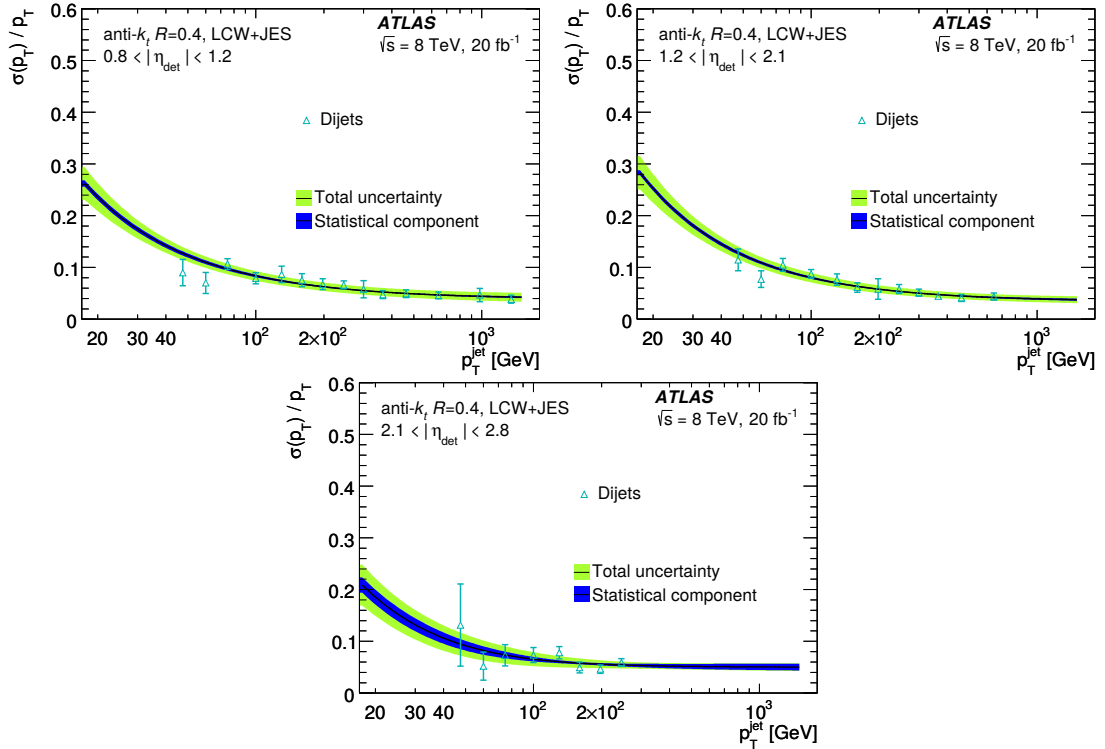
Figure 58: The jet resolution as a function of p_T for LCW+JES anti- k_t , R = 0.4 jets in three more-forward regions. The dijet in situ inputs (empty triangles) to the measurement are shown. The final fit using the function in Eq. (24) is included with its associated statistical and total uncertainty.
