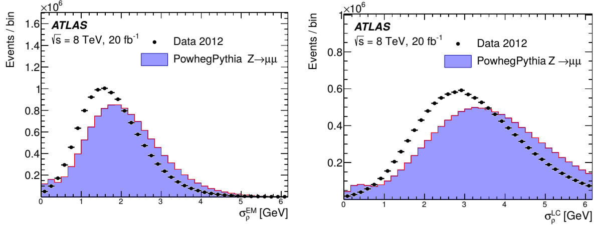
Figure 53: Extracted values of \sigma_\rho in data (points) and MC simulations (histogram) for a sample of Z \rightarrow \mu\mu events at the EM scale (left) and the LCW scale (right). This observable quantifies the fluctuations of the p_T density \rho , i.e. the p_T per area in (y, \phi) -space.
