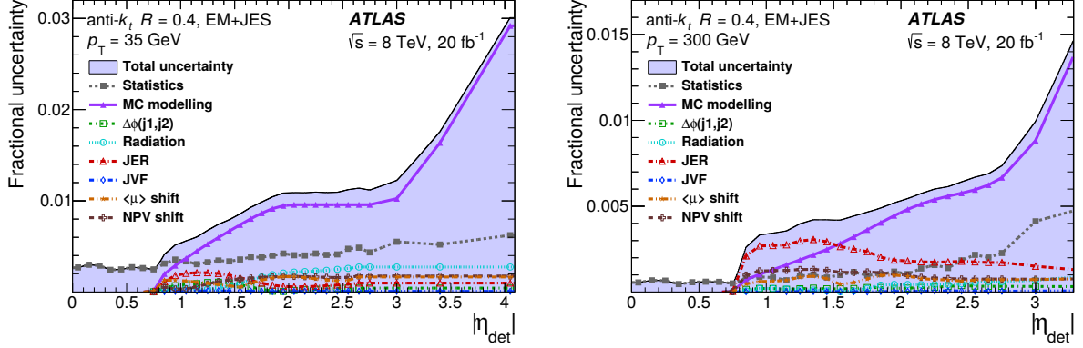
Figure 19: Summary of uncertainties in the intercalibration as a function of the jet \eta_{\text{det}} for anti- k_t jets with R = 0.4 calibrated with the EM+JES scheme, separately for p_T = 35 GeV (left) and p_T = 300 GeV (right). The individual components are added in quadrature to obtain the total uncertainty. The MC modelling uncertainty is the dominant component for jets with |\eta_{\text{det}}| > 1.5 .
