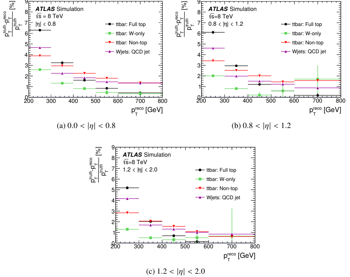
Figure 47: One minus the jet p_T response ( \langle p_T^{\text{truth}} - p_T^{\text{reco}} \rangle / p_T^{\text{truth}} = 1 - \mathcal{R}_{p_T} ) for anti- k_t , R = 1.0 trimmed jets with different flavour composition for (a) 0.0 < |\eta| < 0.8 , (b) 0.8 < |\eta| < 1.2 , (c) 1.2 < |\eta| < 2.0 . The categories in the plot are defined by (1) “ t\bar{t} full top” jets (circles) that represent jets for which the three quarks from a hadronic top quark decay are contained within \Delta R = 0.8 of the jet axis; (2) “ t\bar{t} W-only” jets (squares), for which the quarks from the W boson decay are within \Delta R = 0.8 of the jet axis while the b -quark fulfils \Delta R > 1.2 ; (3) “ t\bar{t} non-top” jets (lower triangles) that represent jets for which the top quark is \Delta R > 2.0 from the jet; and, (4) “Wjets QCD” jets (upper triangles) representing jets from a leptonically decaying W boson in a W +jets MC sample. These are plotted as a function of reconstructed jet p_T ( p_T^{\text{reco}} , but due to the large bin size compared with the p_T resolution, the choice of plotting p_T^{\text{reco}} or p_T^{\text{truth}} is of little significance).
