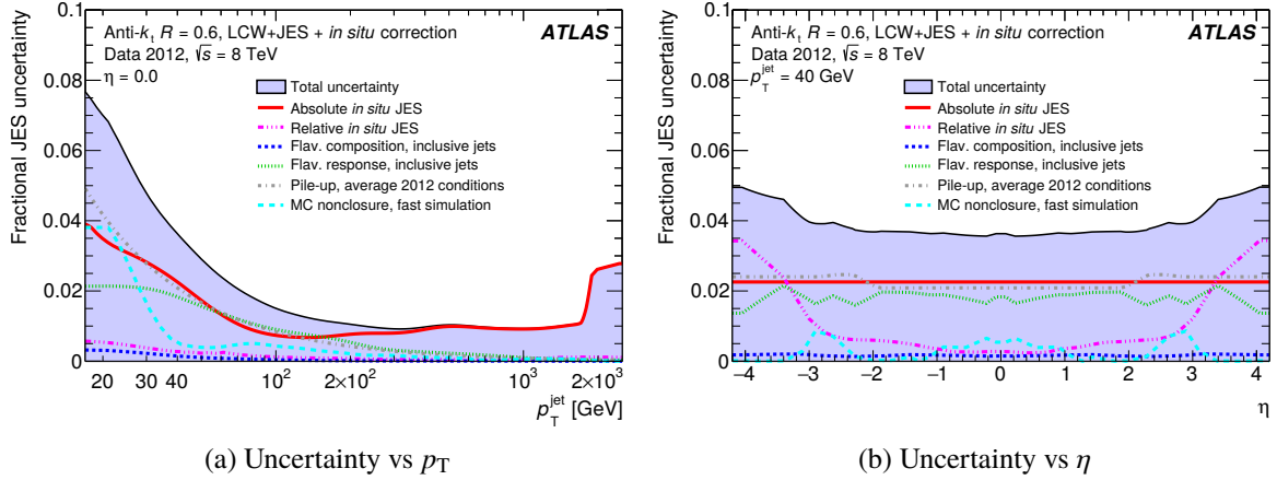
Figure 45: Total uncertainty in the calibration of anti- k_t , R = 0.6 jets in fast simulation as a function of p_T and \eta . The large “MC non-closure” term demonstrates the limitations of using R = 0.6 jets in fast simulation. “Absolute in situ JES” refers to the uncertainty arising from Z +jet, \gamma +jet, and multijet measurements. “Relative in situ JES” refers to the uncertainty arising from the dijet \eta intercalibration.
