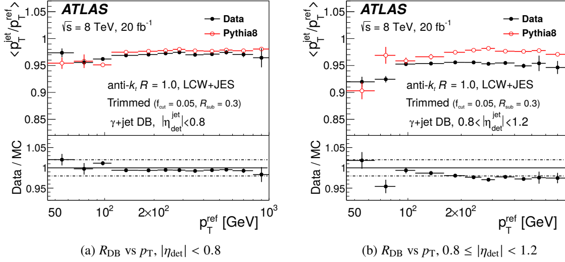
Figure 29: R_{DB} for trimmed anti- k_t jets with R = 1.0 calibrated with the LCW+JES scheme for (a) |\eta_{det}| < 0.8 and (b) 0.8 \leq |\eta_{det}| < 1.2 for both data (filled circles) and MC simulation (empty circles), as a function of the p_T^{ref} . Only statistical uncertainties are shown.
